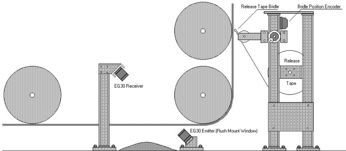
Release Tape Centerguide with Feed Forward Control
